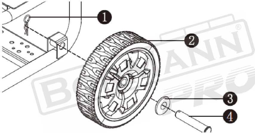
1. Clamp 2. Wheel 3. Washer 4. Wheel stop pin
